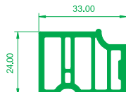
4402 Thermal Insert For 4003 Medium Sash
