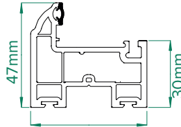
4002 Small Sash
