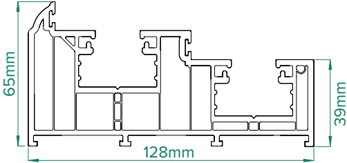
4001 Outerframe
